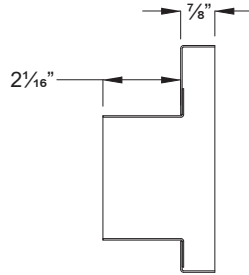
Square/Rectangular Collar Detail
